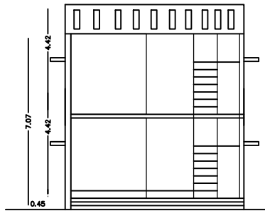
FRONT ELEVATION
