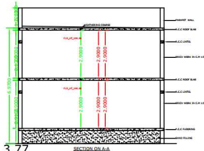
SECTION ON A-A
