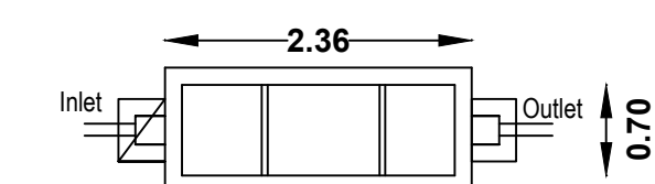
PLAN OF SEPTIC TANK
