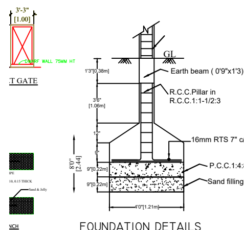
FOUNDATION DETAILS
