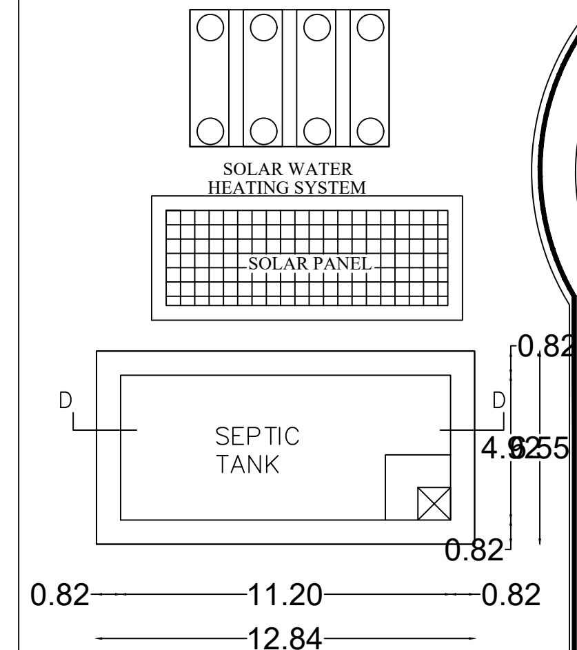
PLAN OF SEPTIC TANK SCALE 1"=2'0"
