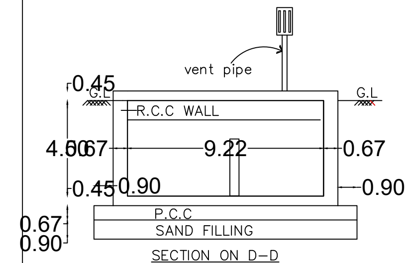
SECTION ON D-D
