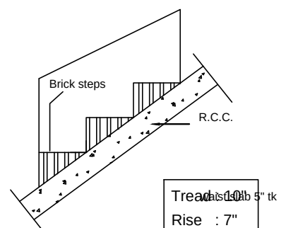
STAIRCASE DETAILS-nts
