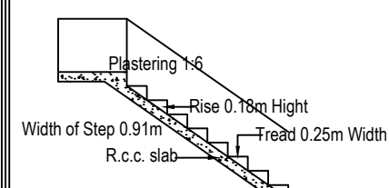
DETAILS OF STAIR CASE
