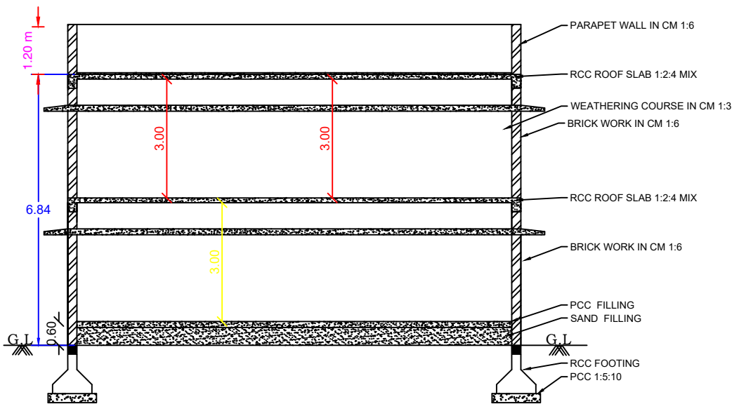
SECTION
