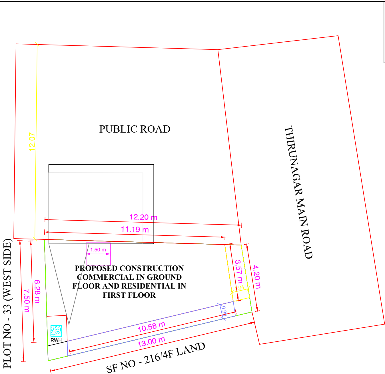
SITE PLAN
