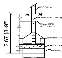
FOUNDATION DETAILS
