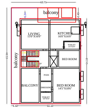
EXG & PRO FIRST FLOOR PLAN
