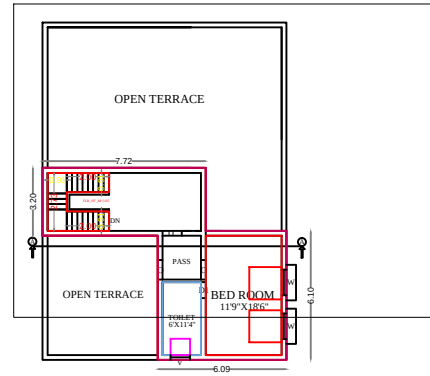
PRO. SECOND FLOOR PLAN
