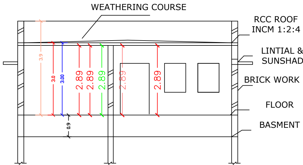
CROSS SECTION 'AB'
