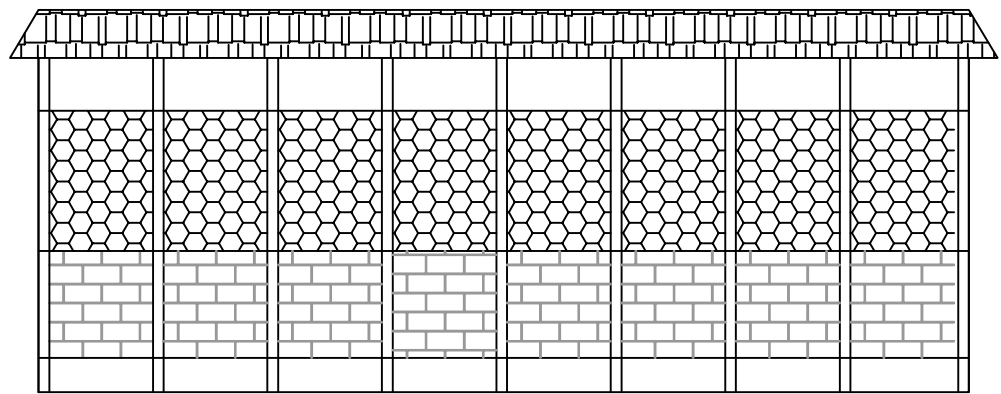
ELEVATION 19,82
