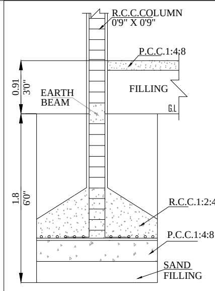
FOUNDATION DETAILS
