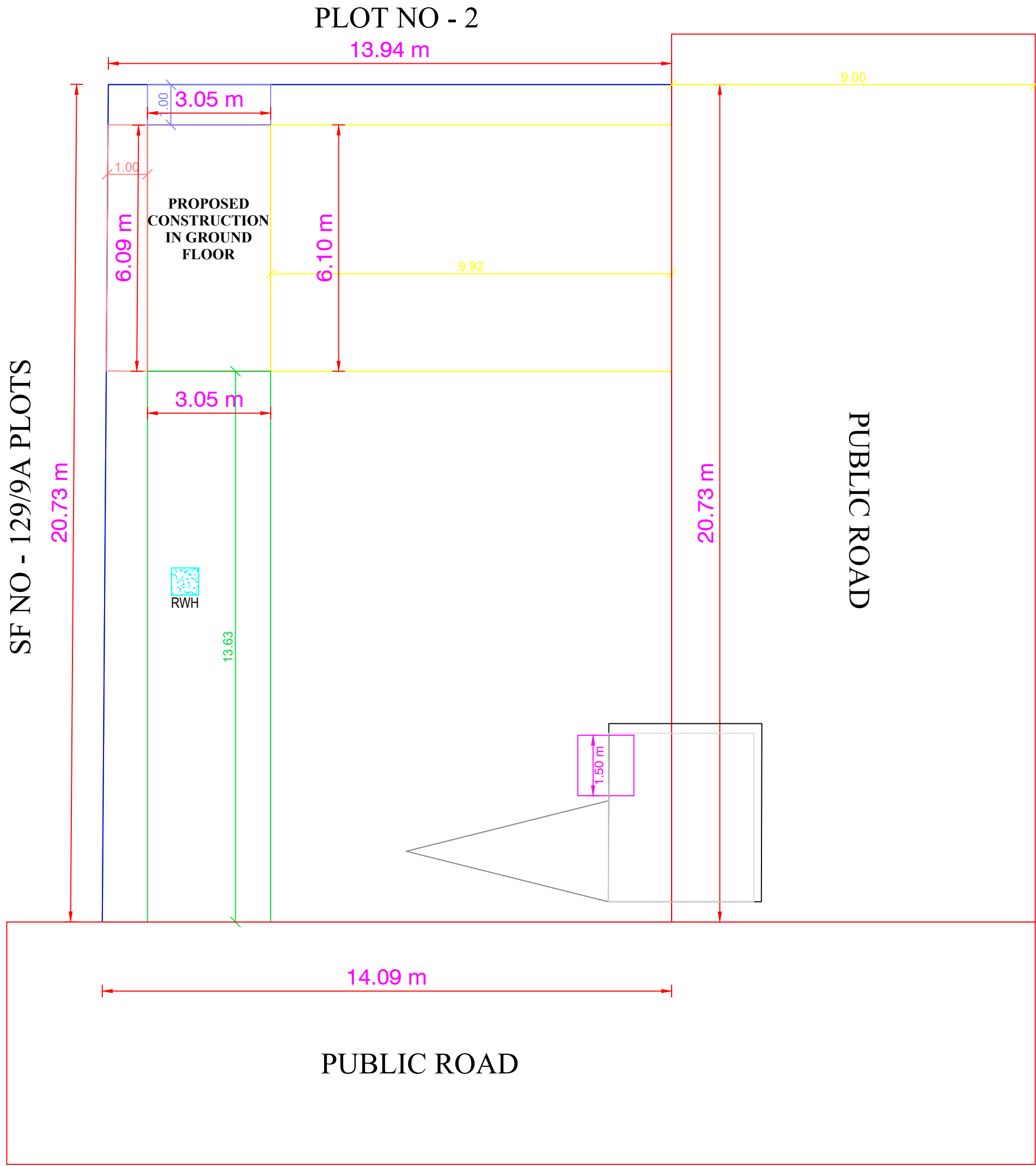
SITE PLAN
