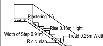
DETAILS OF STAIR CASE
