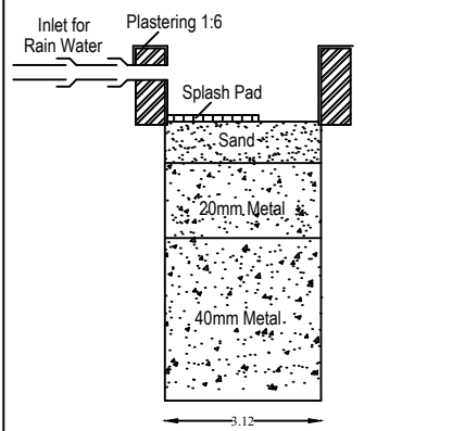
RAIN WATER PERCOLATION PIT
