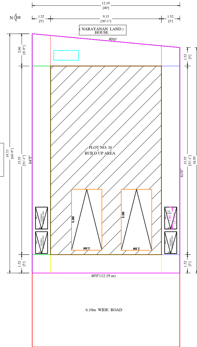
SITE PLAN
