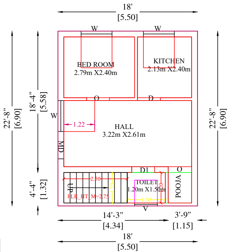
PRO. ROUND FLOOR PLAN
