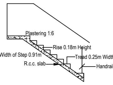
DETAILS OF STAIR CASE
