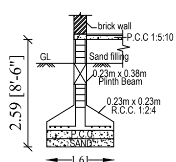
FOUNDATION DETAILS
