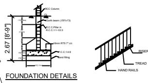
FOUNDATION DETAILS
