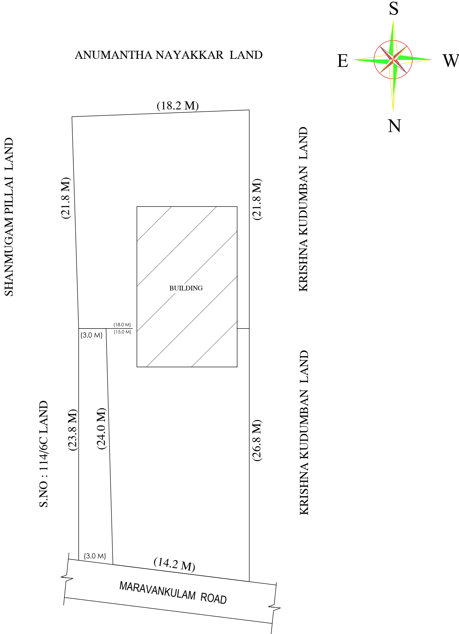
SITE PLAN
