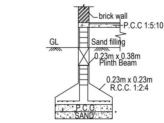
FOUNDATION DETAILS
