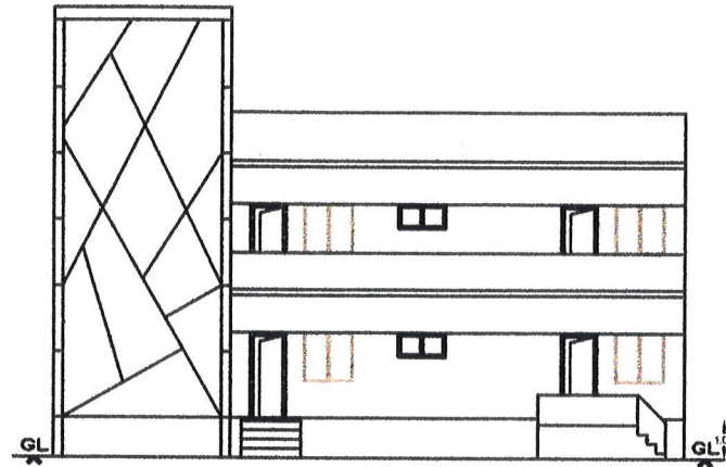
FRONT ELEVATION
