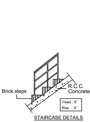
STAIRCASE DETAILS
