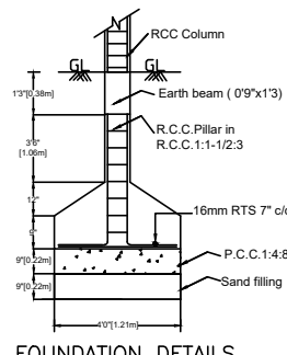
FOUNDATION DETAILS
