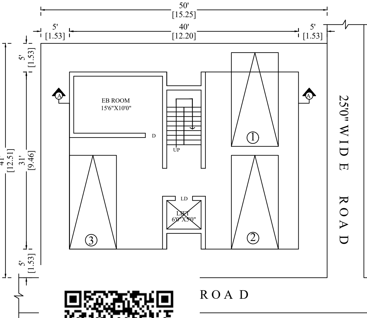
PLAN
