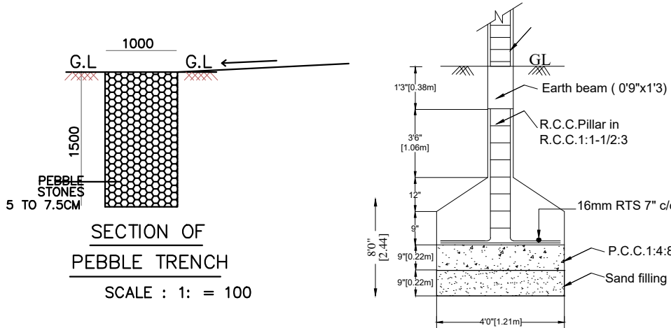
FOUNDATION DETAILS
