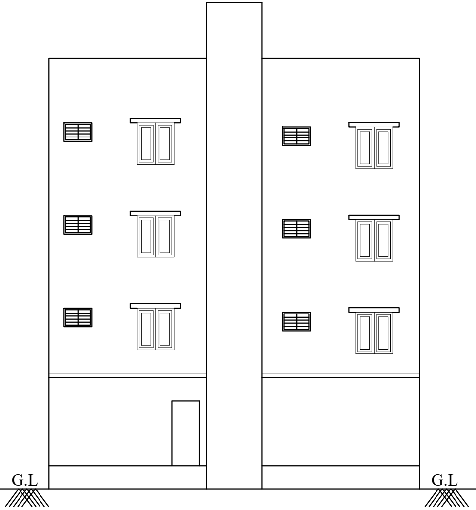
FRONT ELEVATION
