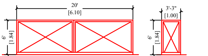
MAIN GATE
