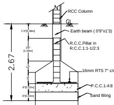
FOUNDATION DETAILS
