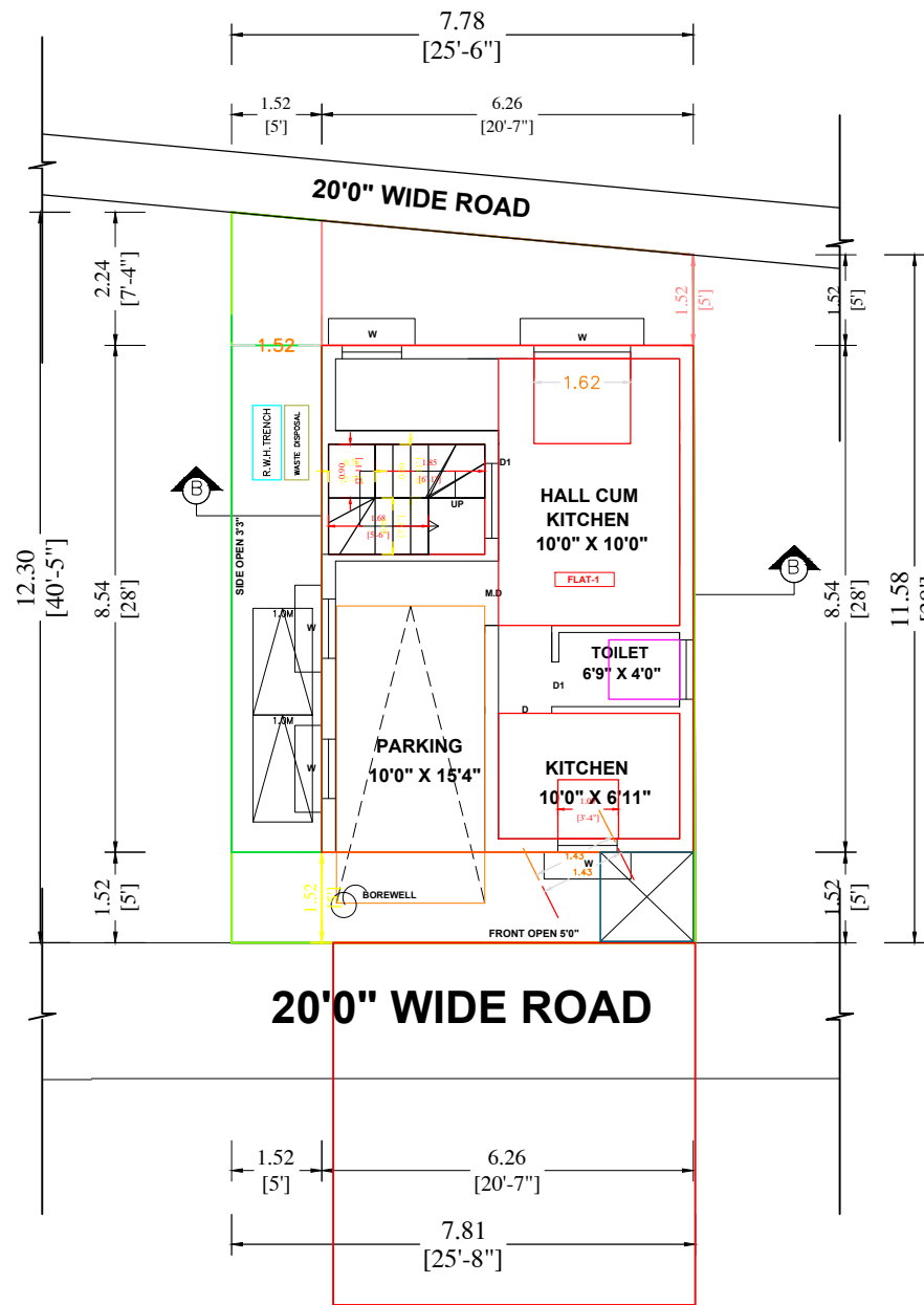
OR PLAN
