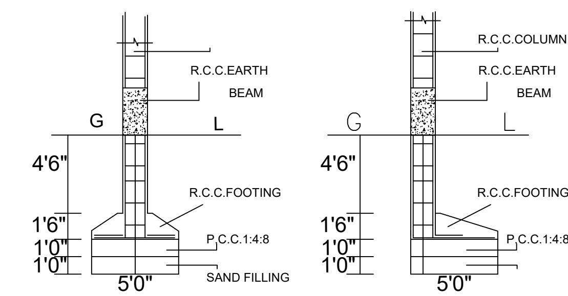
FOUNDATION DETAILS
