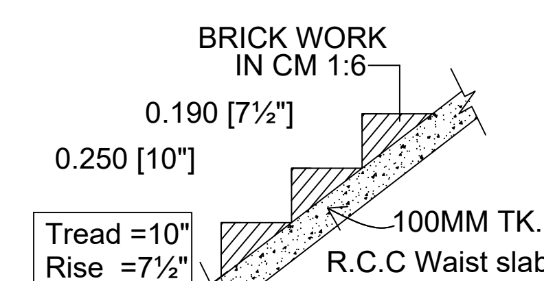
SECTION OF STAIR CASE
