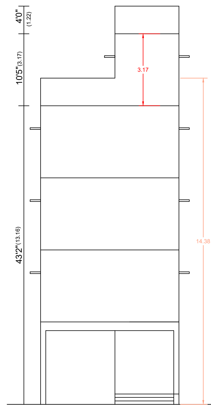
FRONT ELEVATION
