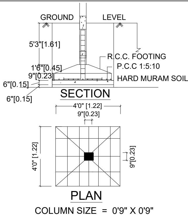
FOUNDATION DETAILS
