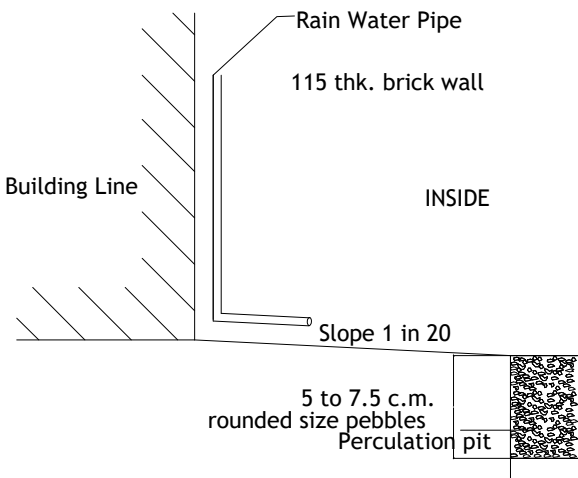
PERCOLATION PIT
