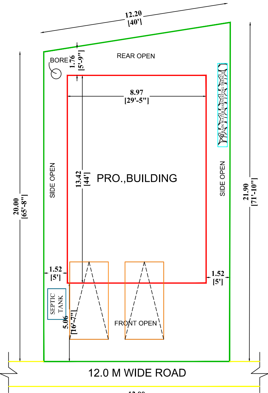
SITE PLAN
