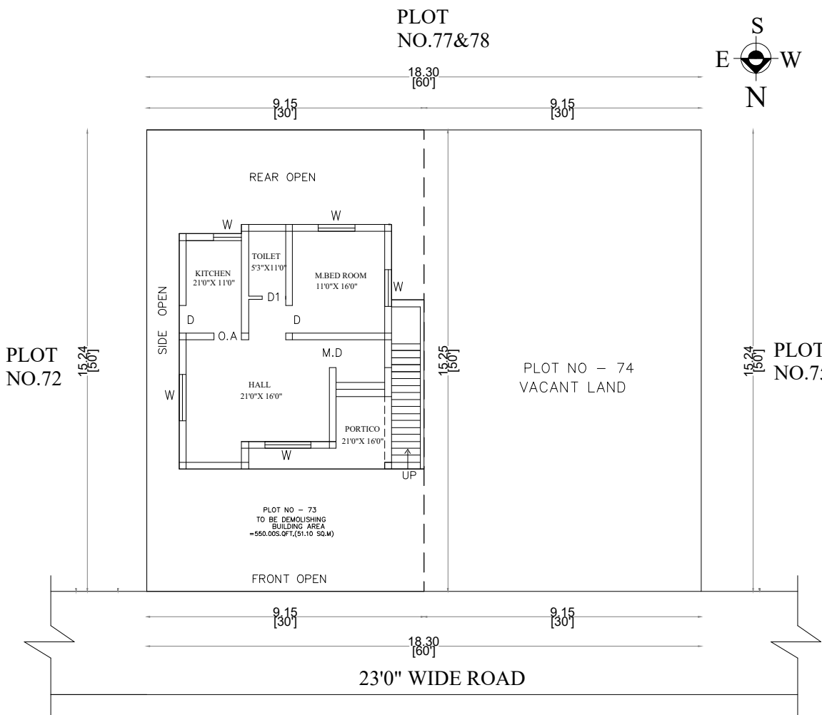
EXG GROUND FLOOR PLAN & SIDE PLAN
