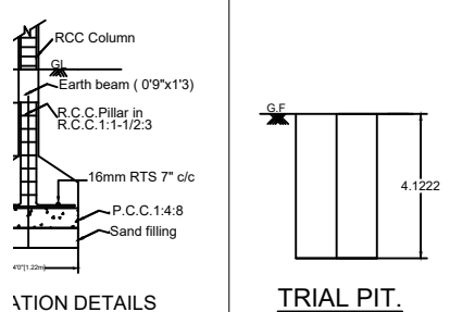
SECTION DETAILS
