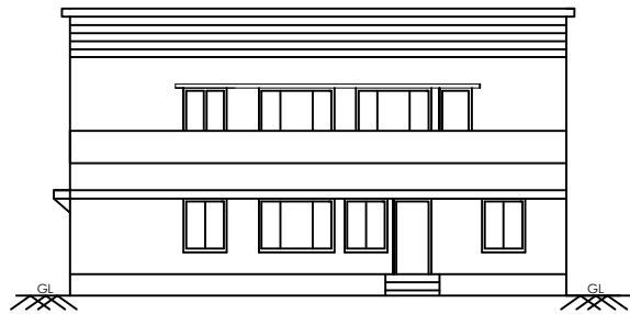
FRONT ELEVATION
