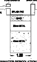
RAINWATER PERCOLATION PIT
