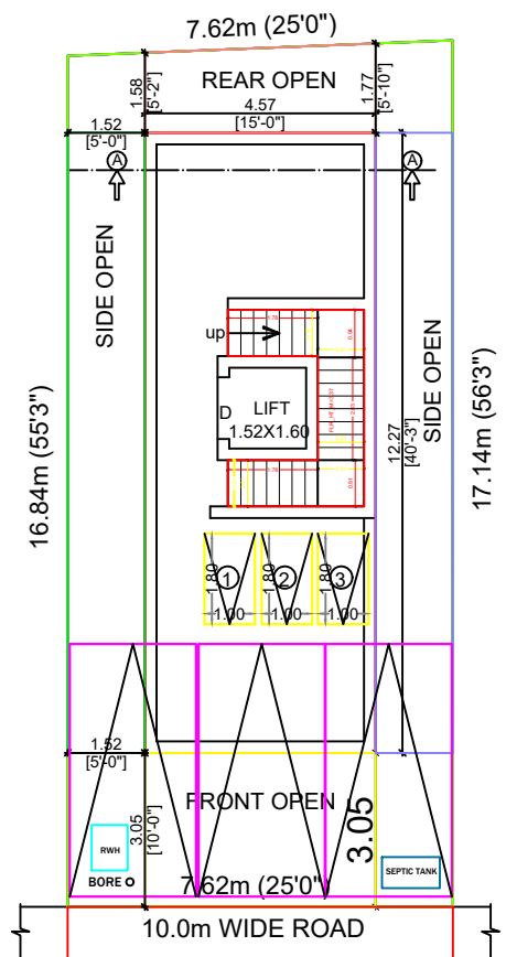
SITE PLAN AND STILT FLOOR PLAN (PROPOSED)
