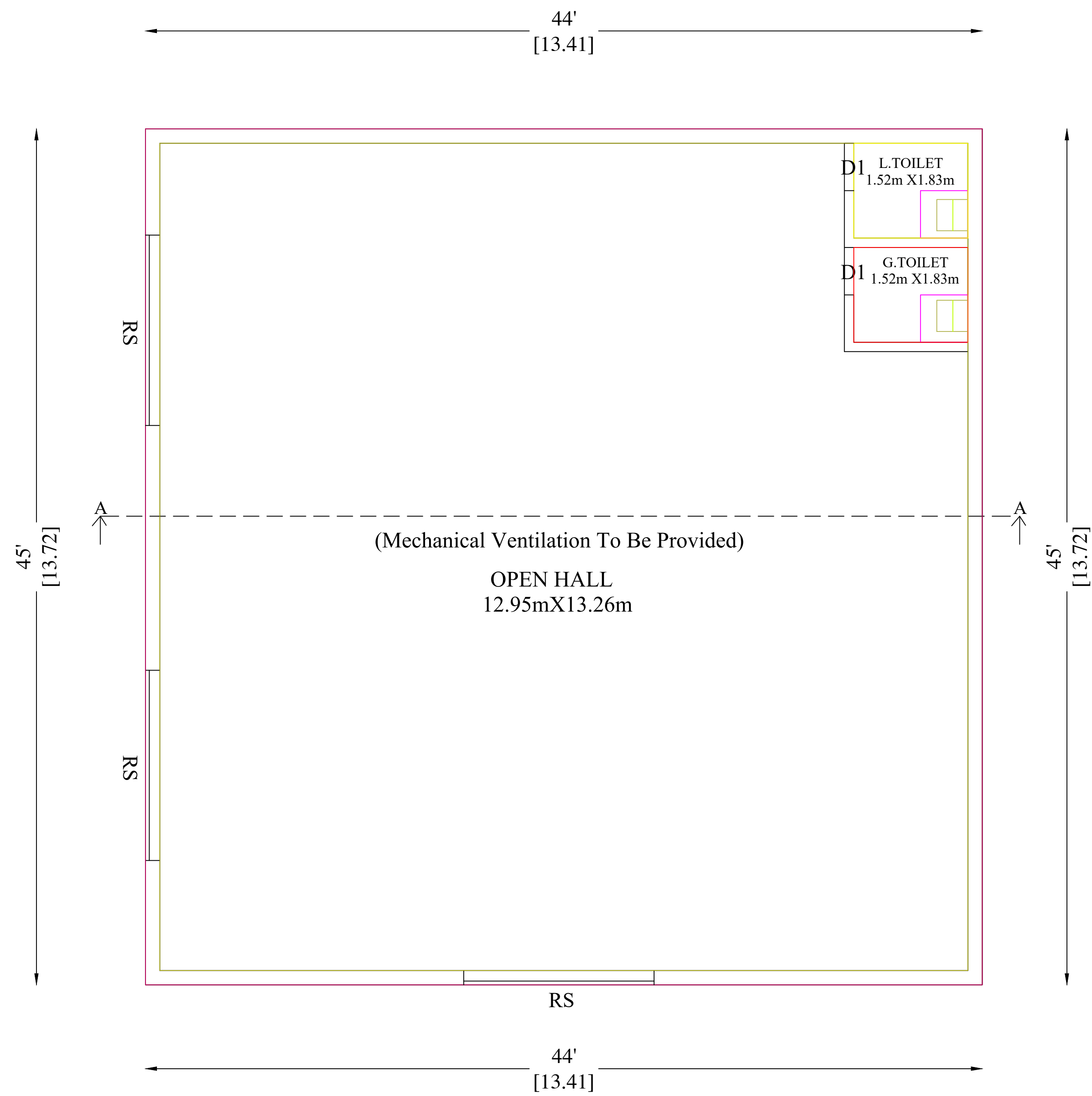
PRO. GROUND FLOOR PLAN
