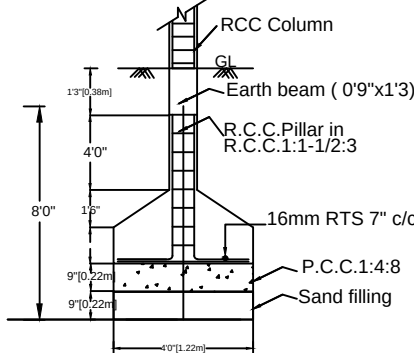
FOUNDATION DETAILS
