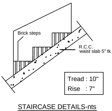
STAIRCASE DETAILS-nts
