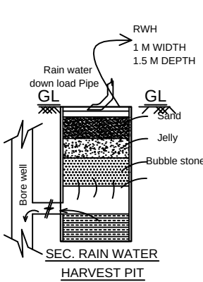
SEC. RAIN WATER HARVEST PIT
