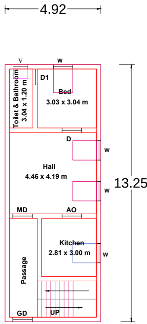
Ground Floor Plan South facing
