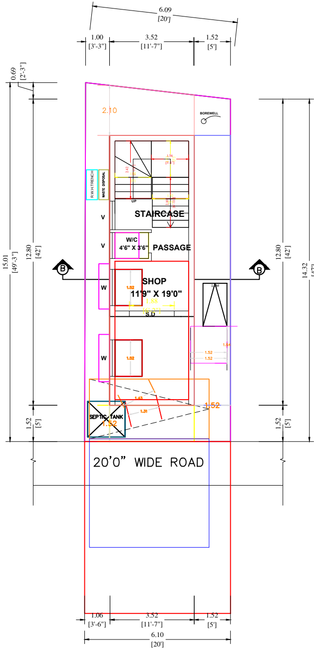
GROUND FLOOR PLAN EXISTING
