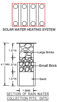
SECTION OF RAIN WATER COLLECTION PITS (NTS)
