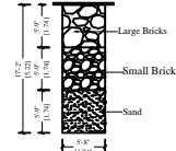
SECTION OF RAIN WATER COLLECTION PITS (INTS)
