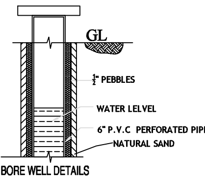
BORE WELL DETAILS
