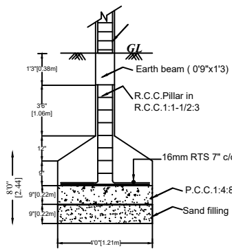
FOUNDATION DETAILS
