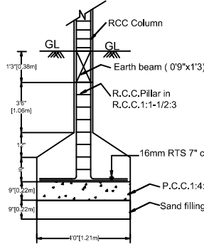
FOUNDATION DETAILS
