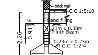
FOUNDATION DETAILS
