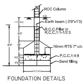
FOUNDATION DETAILS
