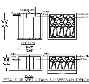
DETAILS OF SEPTIC TANK & DISPERSION TRENCH
