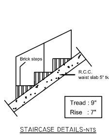
STAIRCASE DETAILS-NTS
