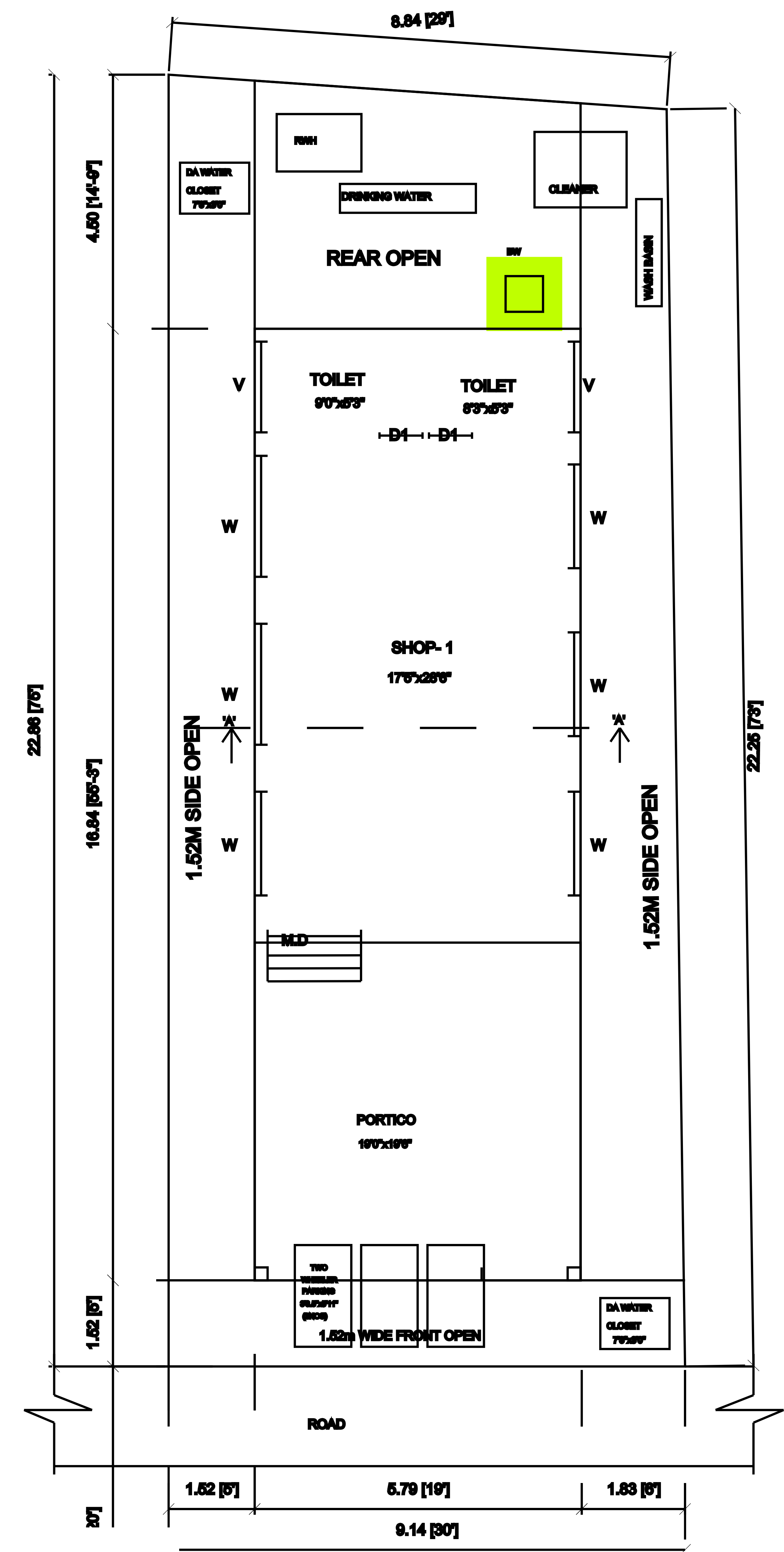
PROPOSED GROUND FLOOR PLAN
