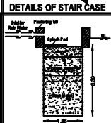
RAIN WATER PERCOLATION PIT
