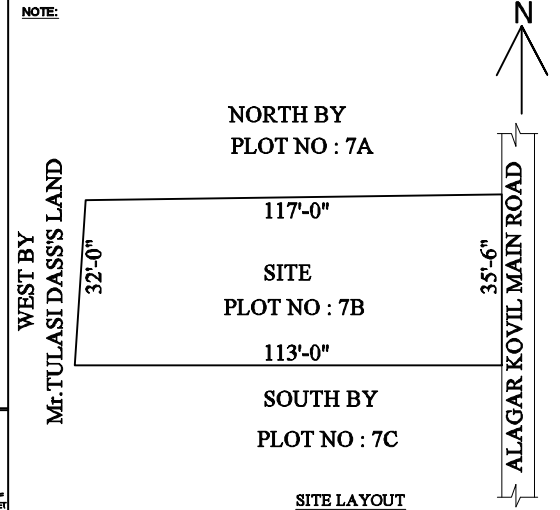
SITE LAYOUT
