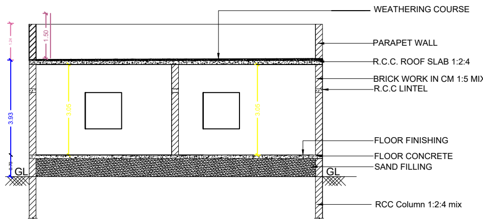
SECTION - 'RI'
