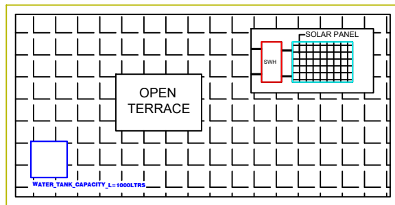
PROPOSED TERRACE FLOOR PLAN
