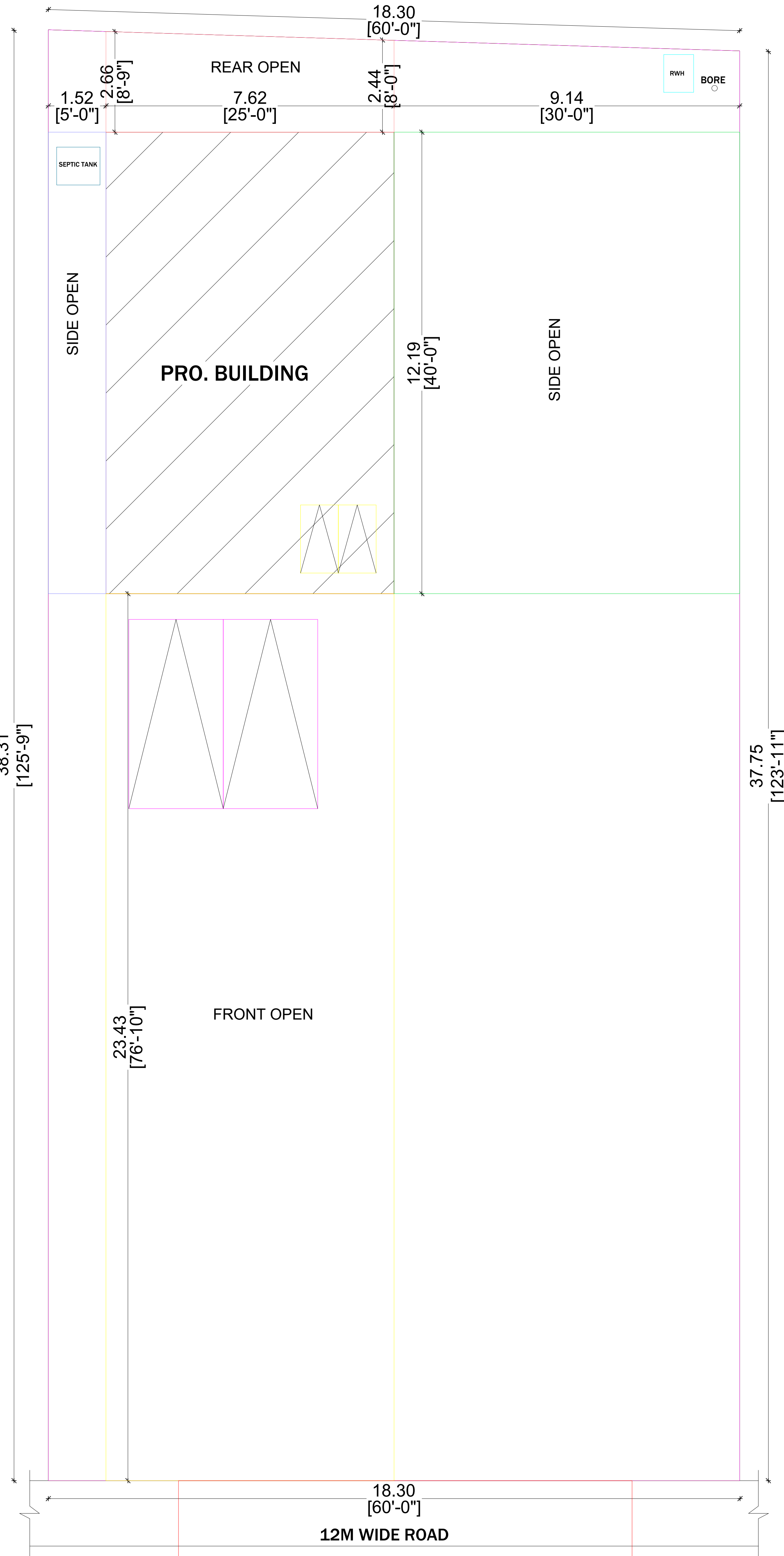
SITE PLAN
