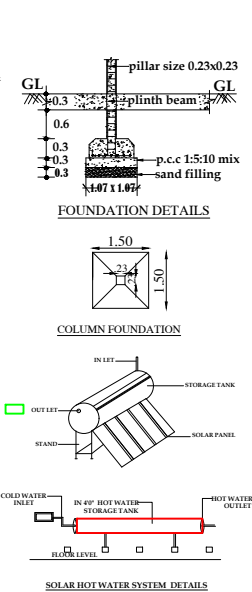
SOLAR HOT WATER SYSTEM DETAILS
