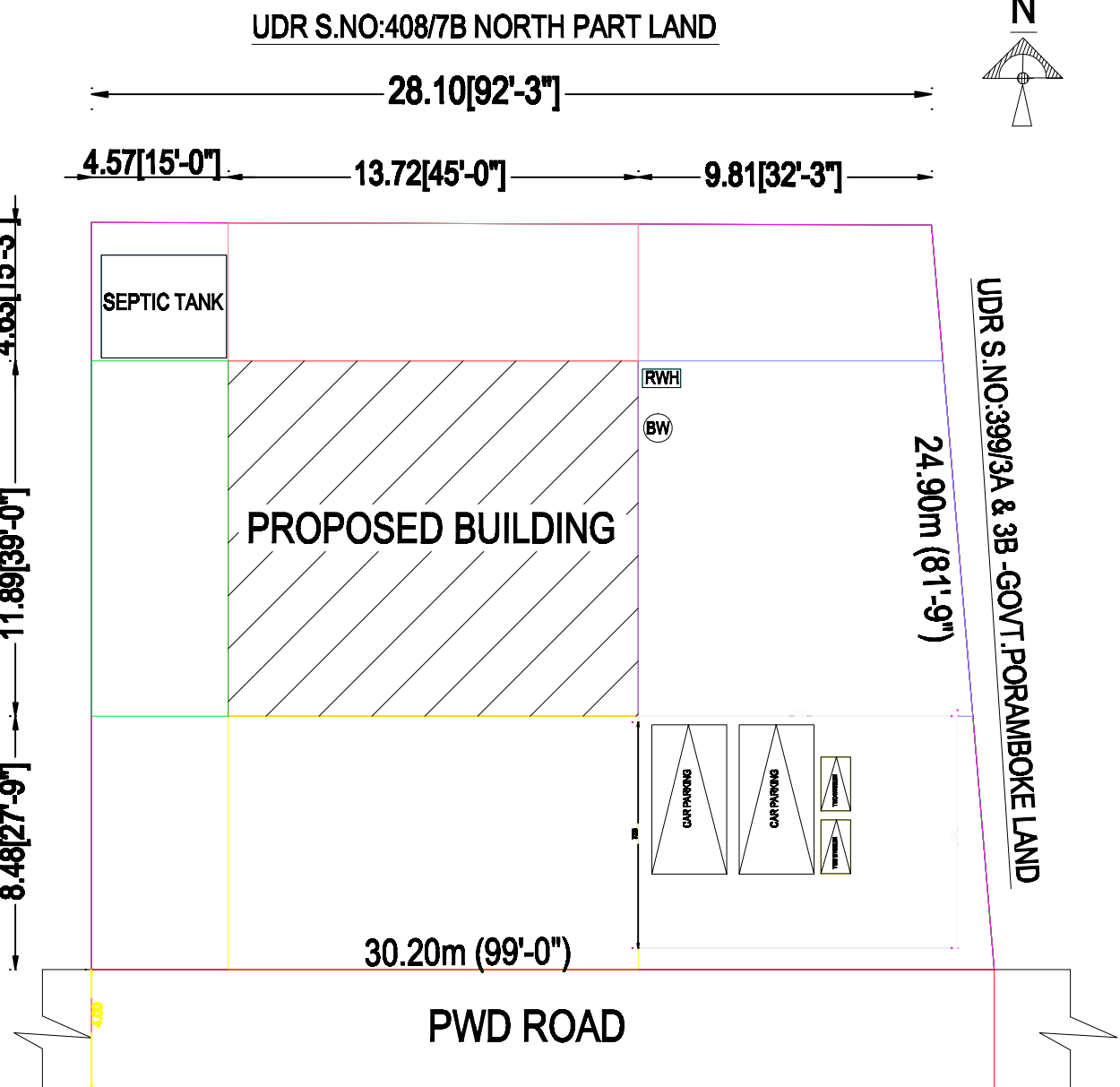
SITE PLAN
