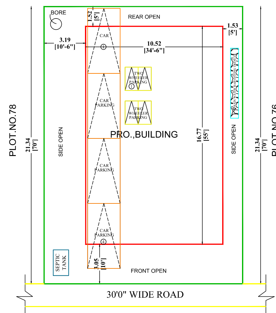
SITE PLAN
