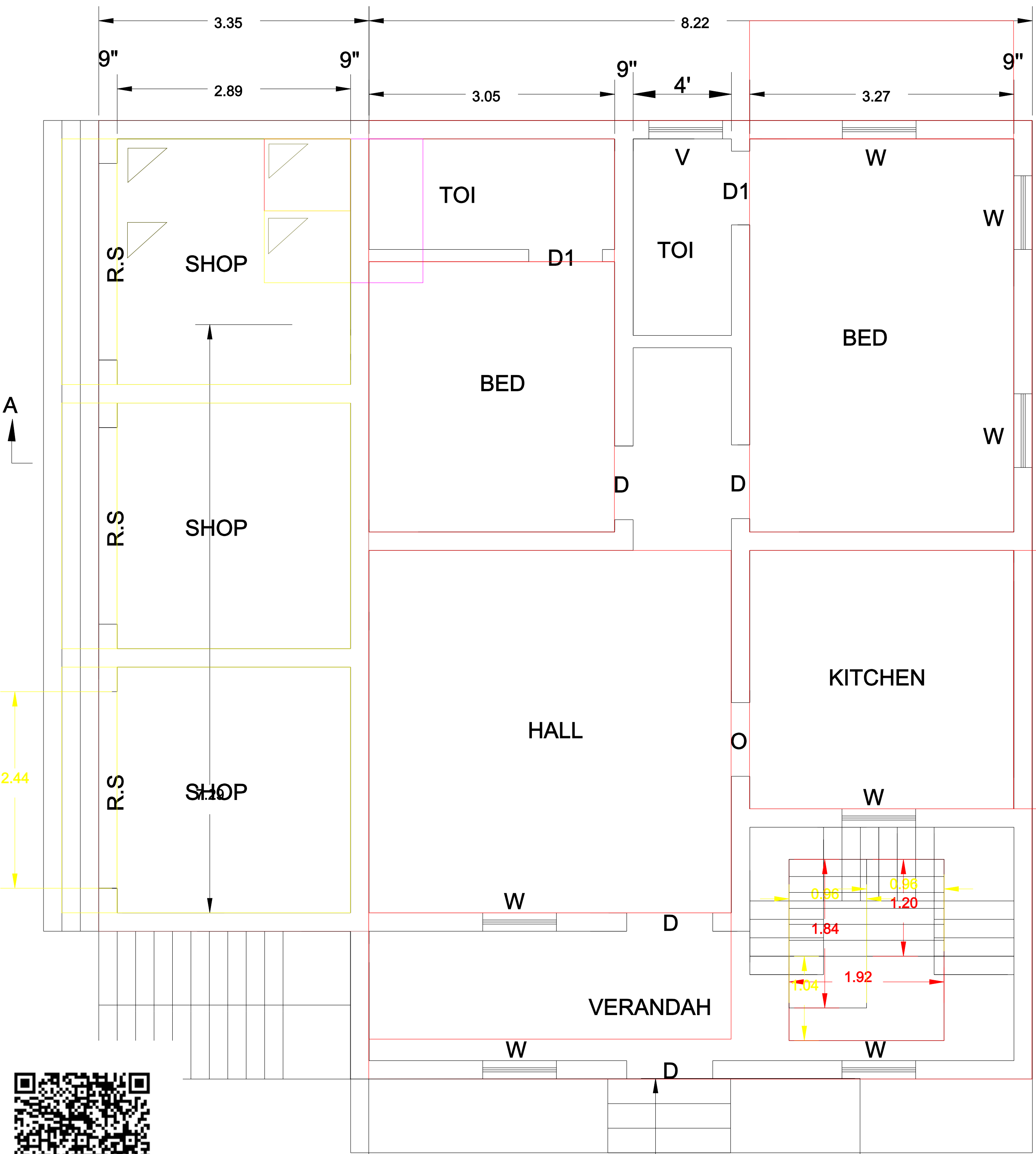
G.F. PLAN
