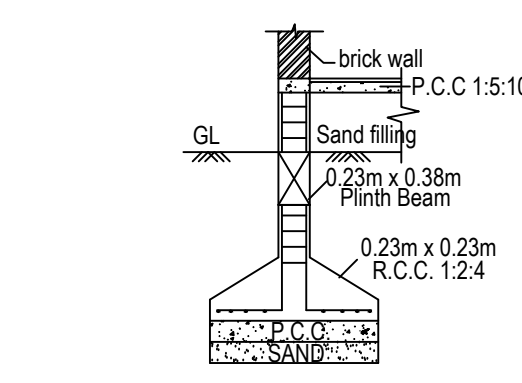
←1.60→ FOUNDATION DETAILS
